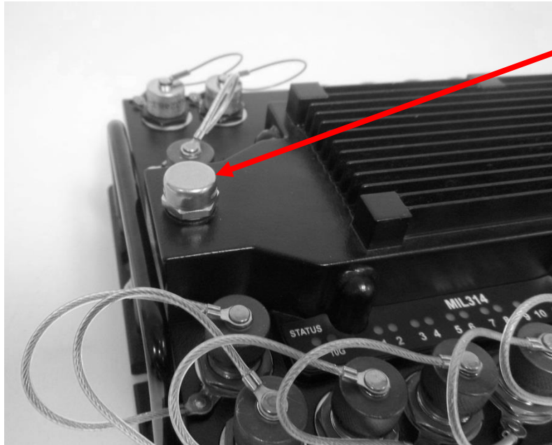
Pressure Vent
