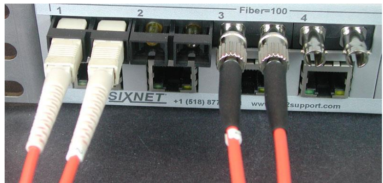
This image shows the fiber cables connected to the ports. The SC snap-in and the ST are a 1/4-turn bayonet style.
