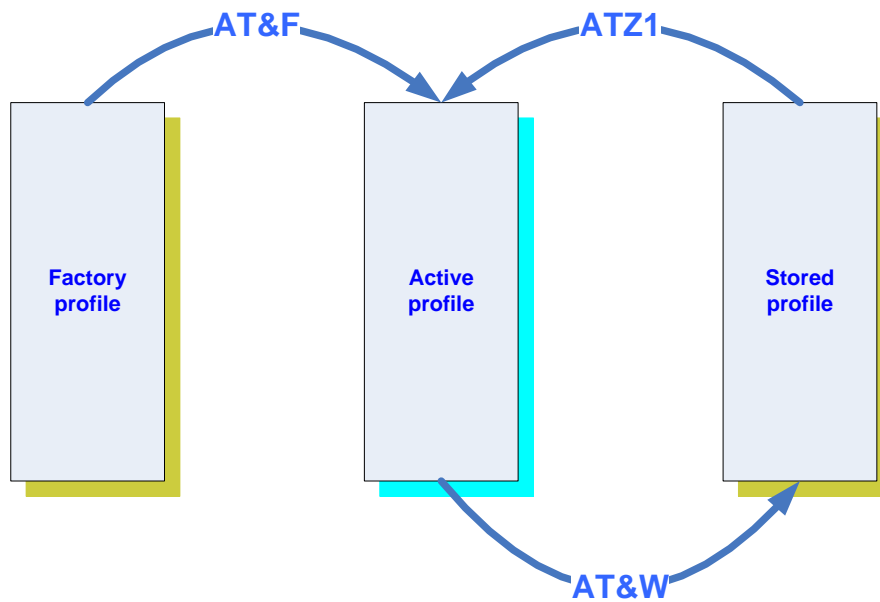
Figure 1: Modem configuration profiles
