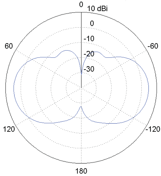
Elevation Pattern
