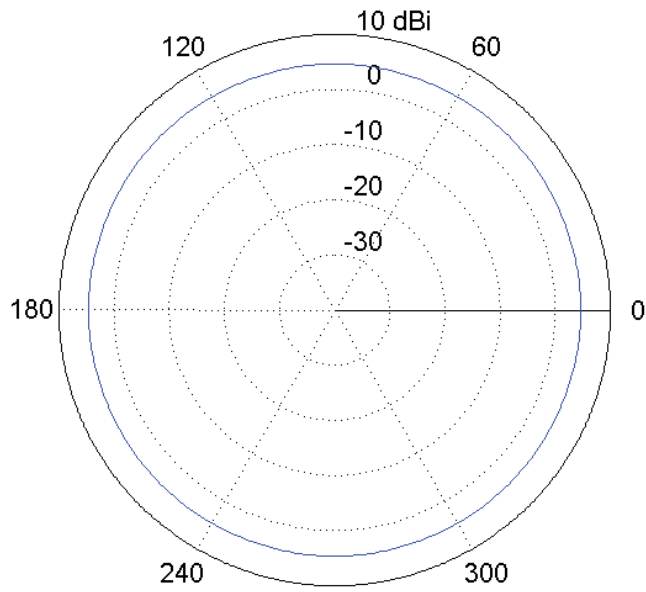
Azimuth Pattern
