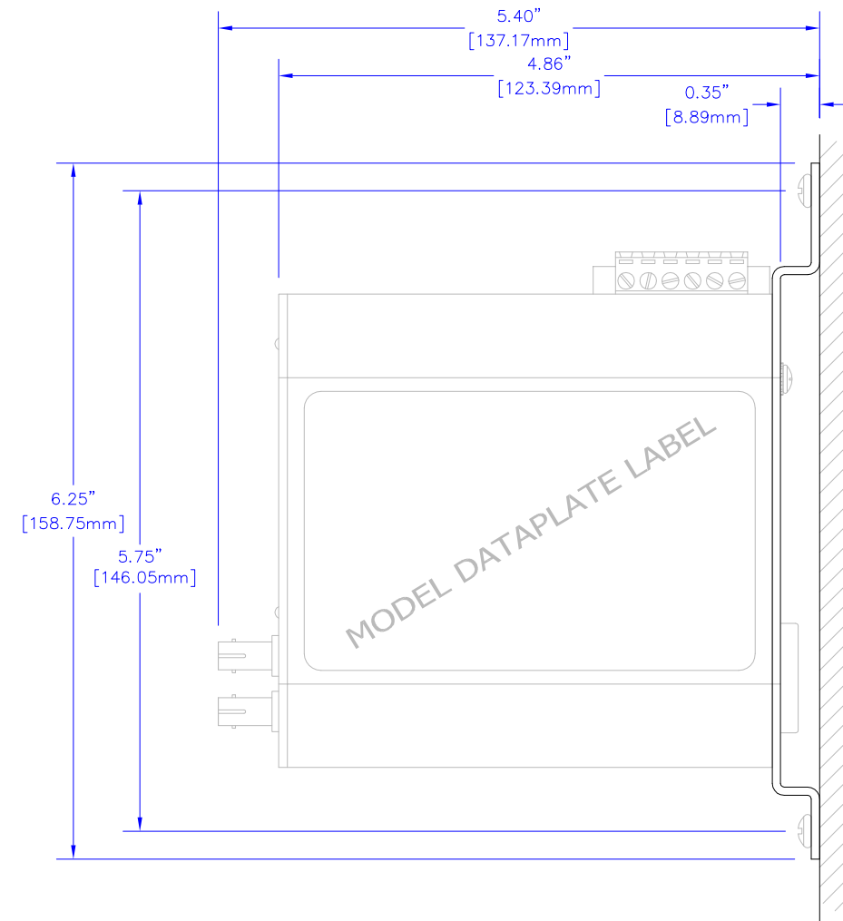
OPTIONAL COMPACT PANEL MOUNT ASSY. ( P/N: CPMA-1 )
