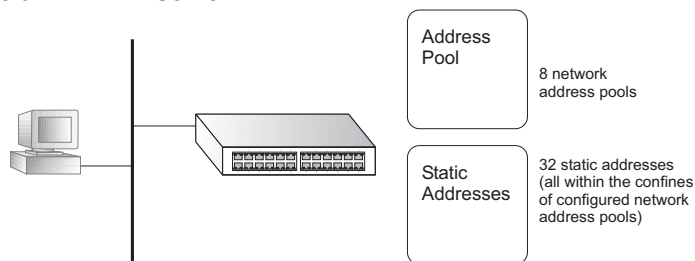
Figure 321: DHCP Server
