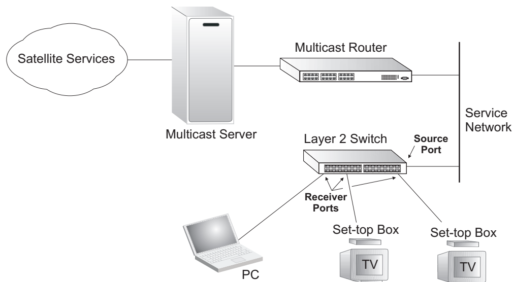
Figure 266: MVR Concept
