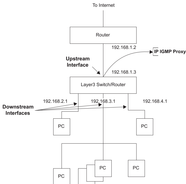
Figure 259: IGMP Proxy Routing
