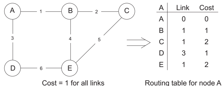
Figure 334: Configuring RIP
