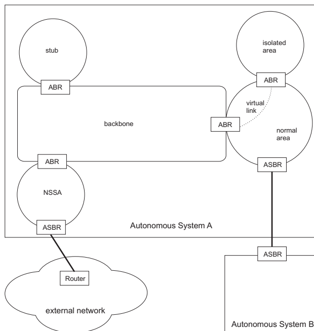
Figure 352: Configuring OSPF
