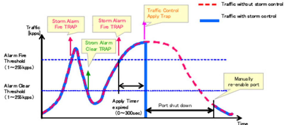
Figure 2: Storm Control by Shutting Down a Port
