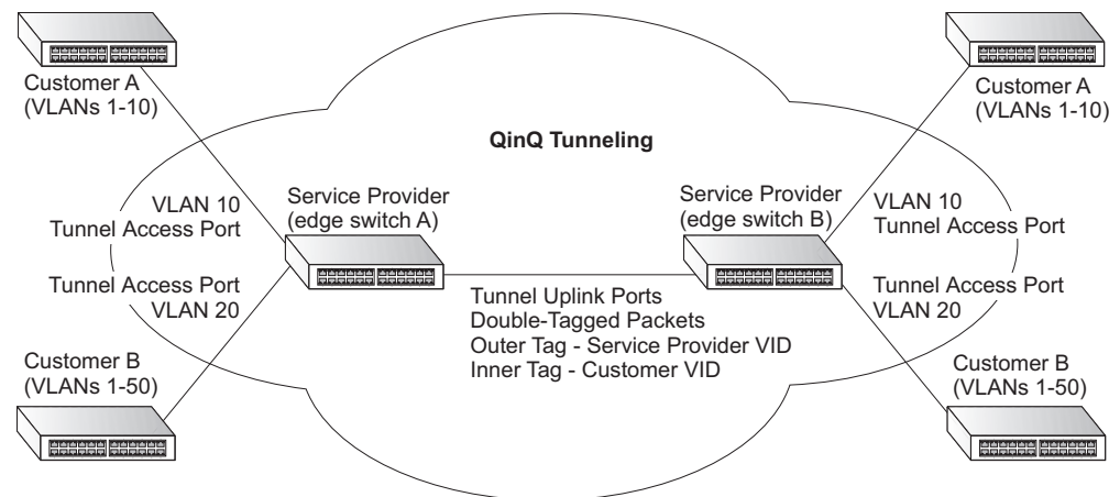
Figure 70: QinQ Operational Concept
