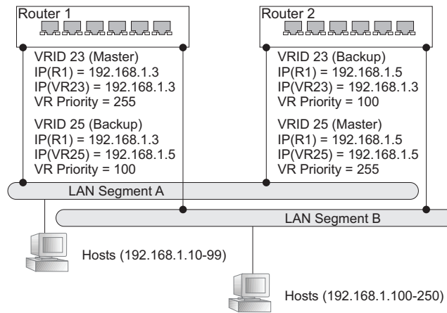
Figure 302: Several Virtual Master Routers Configured for Mutual Backup and Load Sharing
