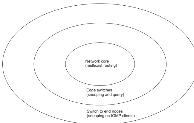
Figure 241: IGMP Protocol
