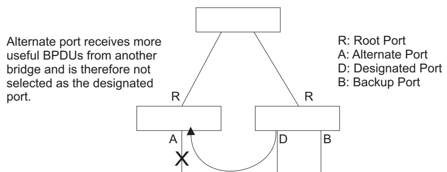
Figure 96: STA Port Roles
