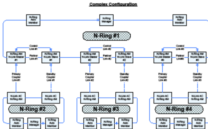
Example of a complex N-Link configuration
