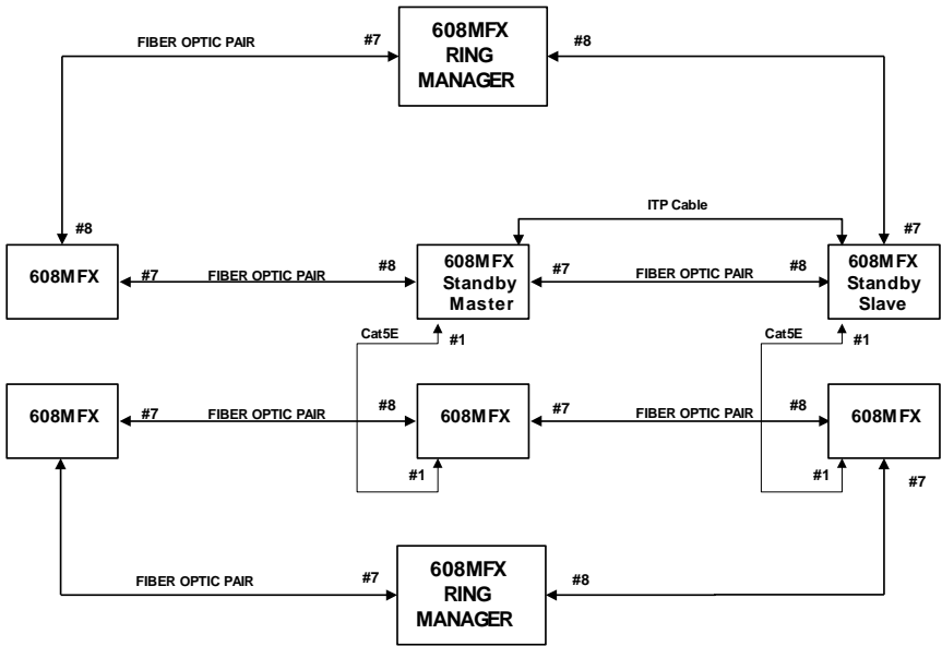
608MFX Network Segment Redundancy Figure 2
