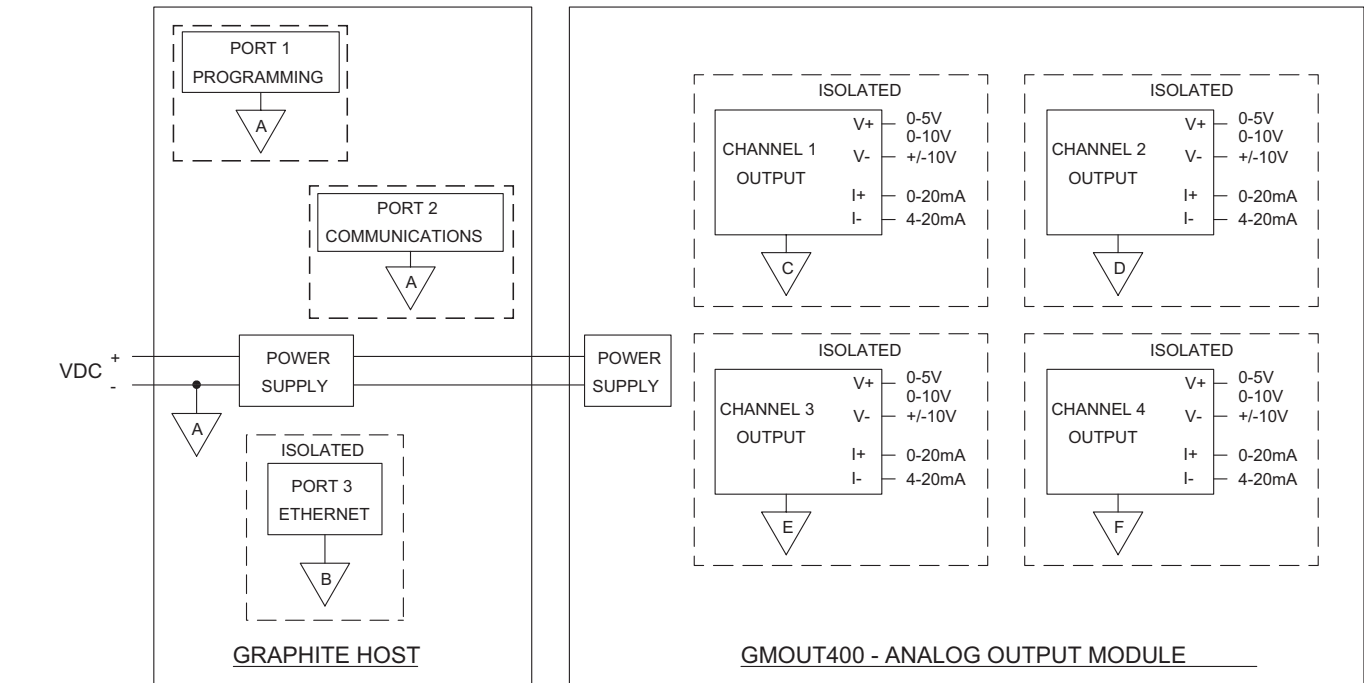
Block Diagram for GMOUT
