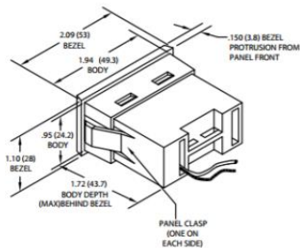
CUB3 Rear View
