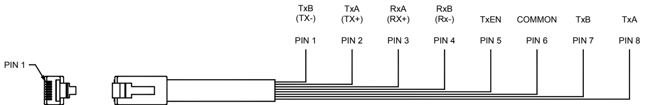
CBLGEN03 - RS485
