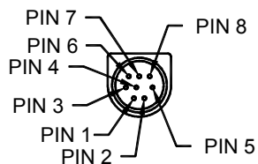
MINI-DIN 8 CONNECTOR
