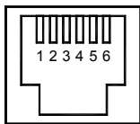
RS232 PORT (FROM RLC UNIT)
