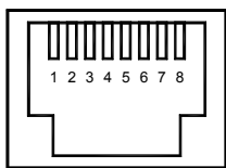
RS485 PORT (FROM RLC UNIT)
