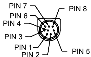
MINI-DIN 8 CONNECTOR
