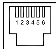
RS485 PORT - RJ11 (FROM RLC UNIT)
