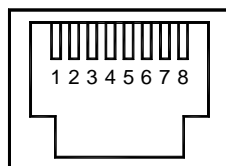
RS485 PORT - RJ45 (FROM RLC UNIT)
