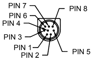
MINI-DIN 8 CONNECTOR
