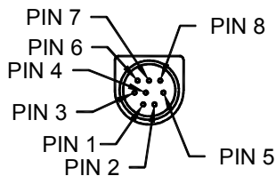
MINI-DIN 8 CONNECTOR
